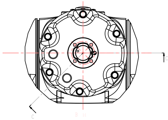
Detailed drawing of end-effector mounting face
