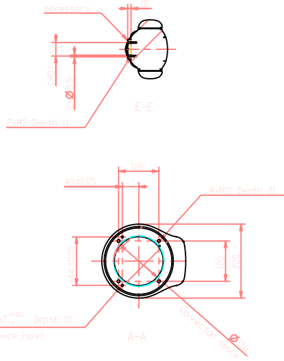
Detailed drawing of base mounting face
