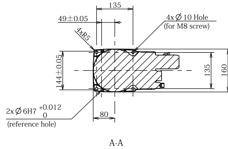
Detailed drawing of base mounting face
