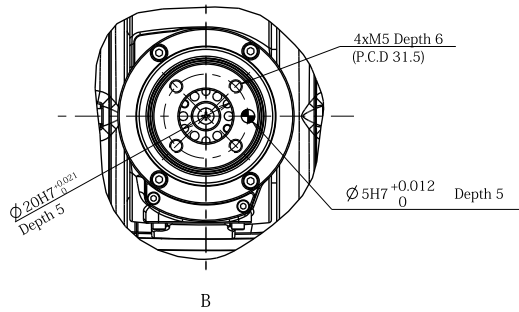
Detailed drawing of end-effector mounting face
